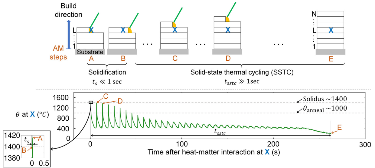
Fig. 1. An illustration of temperature ( \theta ) vs time ( t ) evolution at a material point X during additive manufacturing of a wall. t = 0 corresponds to the moment the heat-matter interactions occur at X in a layer L < N , where N is the total number of layers.
